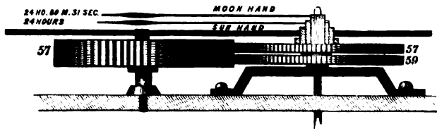
Front Frame of the Clock.
